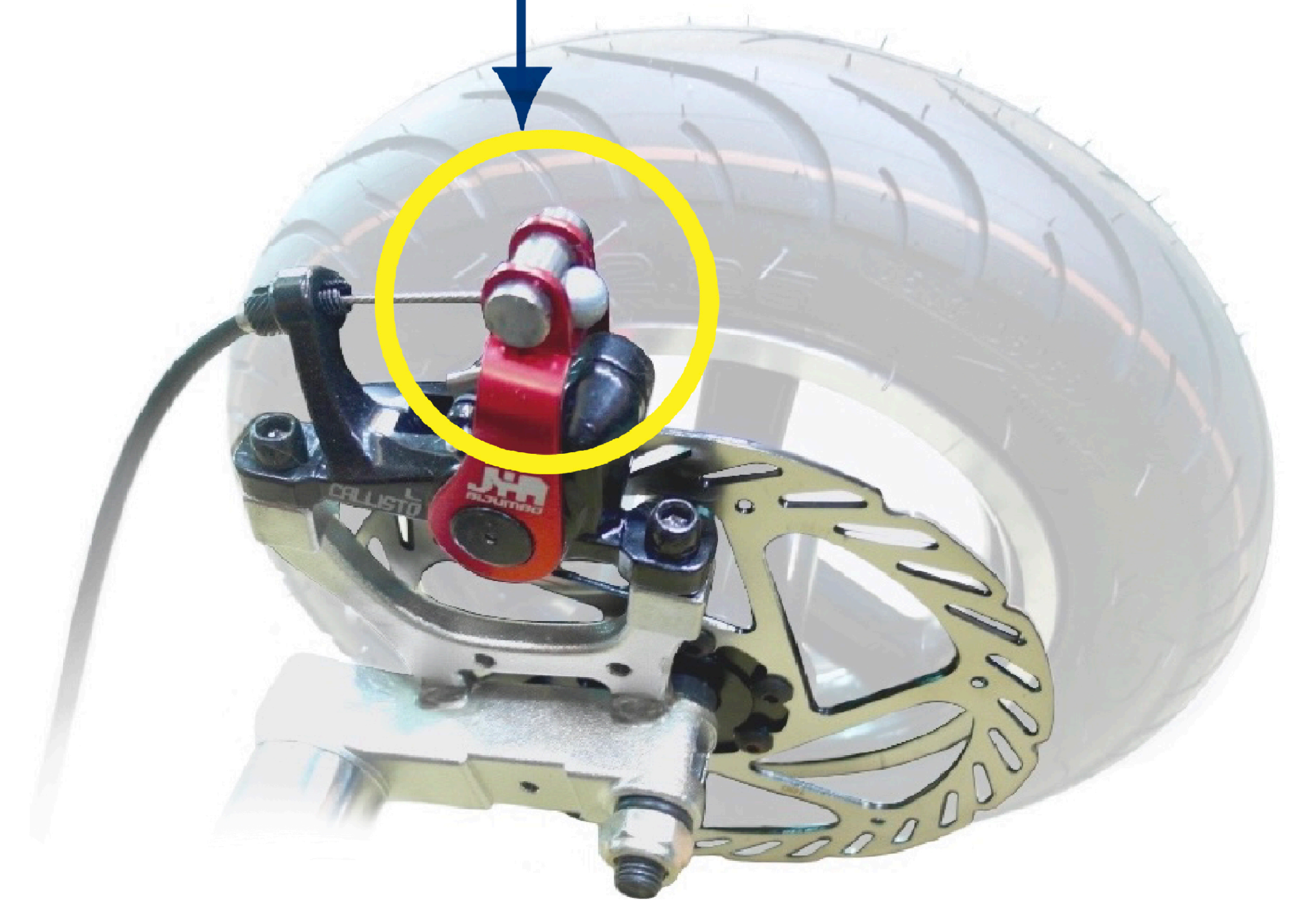
右後輪卡鉗 Right rear wheel calliper
